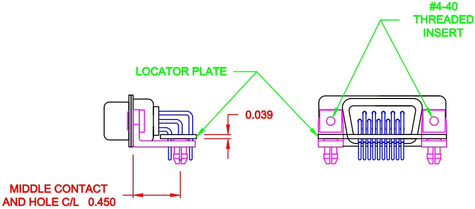
BRACKETS MOUNTED ON CONNECTOR WITH LOCATOR PLATE
