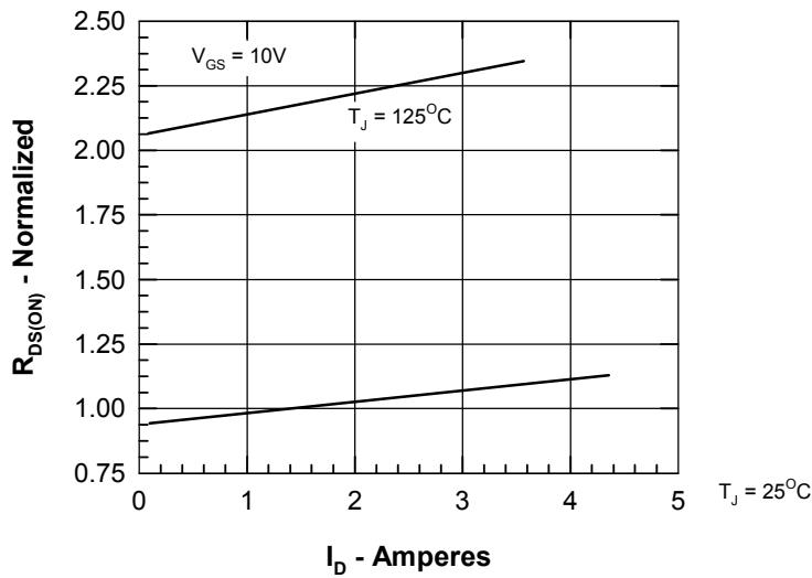
Fig. 3 R_{DS(on)} vs. Drain Current
