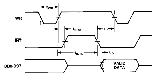
Figure 13. \overline{WR} - \overline{RD} Mode Stand-Alone Operation, \overline{CS} = \overline{RD} = 0
