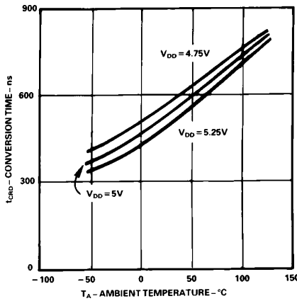
Conversion Time (RD Mode) vs. Temperature
