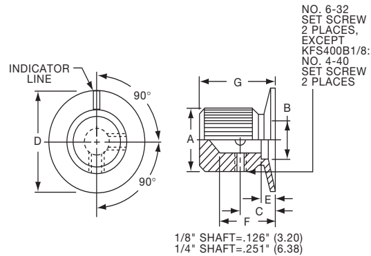
Straight Knurl with Indicator on Skirt
