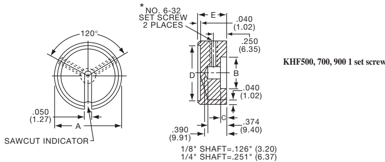
Plain Body with Top and Side Sawcut Indicator
