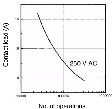
2. Life curve
