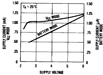
MAX697 SUPPLY CURRENT AS A FUNCTION OF SUPPLY VOLTAGE
