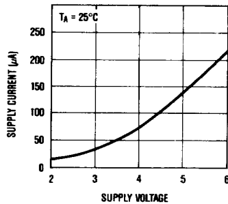
MAX697 SUPPLY CURRENT AS A FUNCTION OF SUPPLY VOLTAGE
