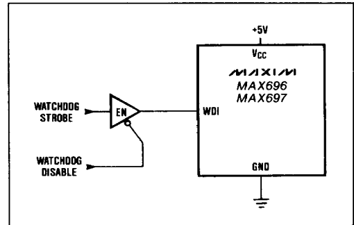
Figure 8. Disabling the Watchdog Under Program Control
