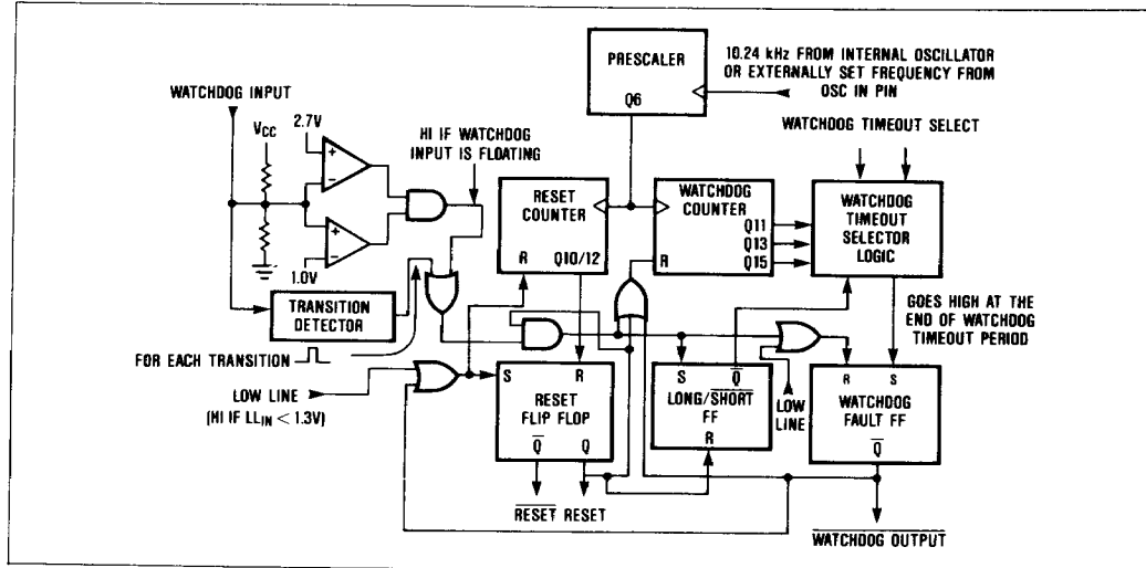
Figure 6. Watchdog Timer Block Diagram
