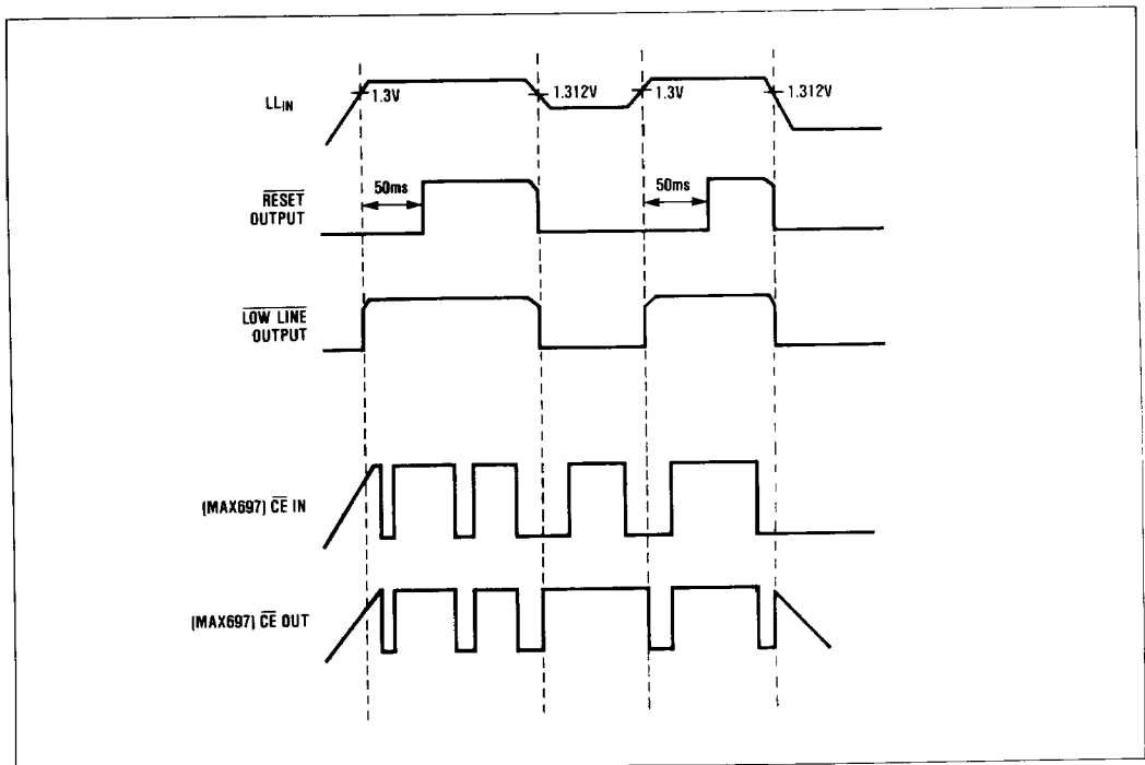
Figure 5. MAX697 Reset Timing
