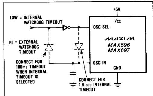
Figure 9. Selecting Internal or External Watchdog Timeout
