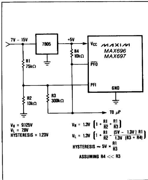
Figure 7. Adding Hysteresis to the Power Fail Voltage Comparator
