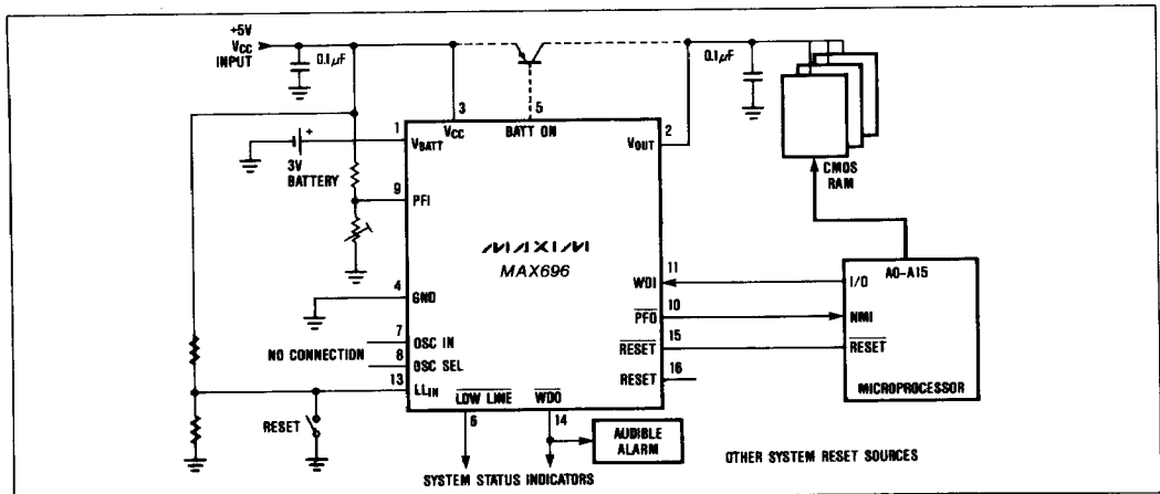
Figure 1. MAX696 Typical Application
