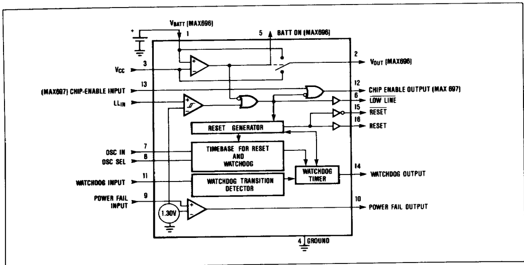
Figure 2. MAX696/697 Block Diagram
