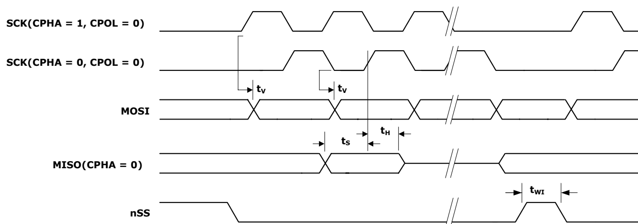
FIGURE 3. SPI TIMING
