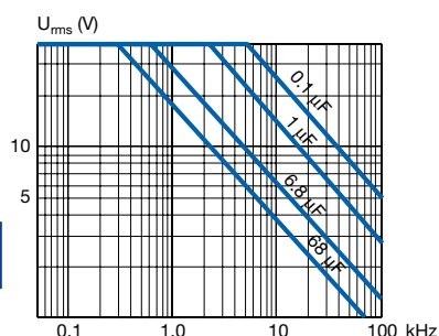
MMK7.5 ... 37.5 63/40
