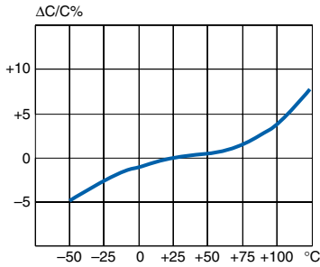
Capacitance vs. temperature (at 1 kHz)
