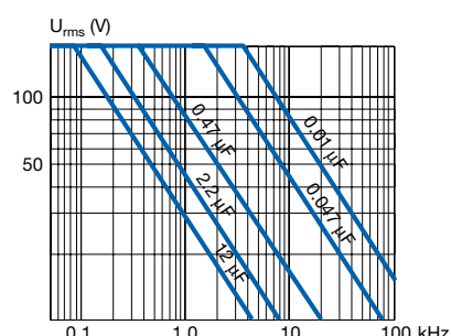
MMK7.5 ... 37.5 250/160
