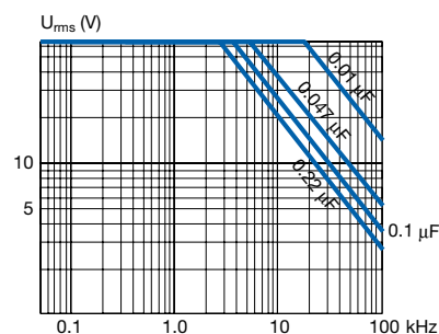
MMK5 100/63
