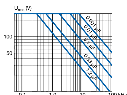
MMK7.5 ... 37.5 1000/250
