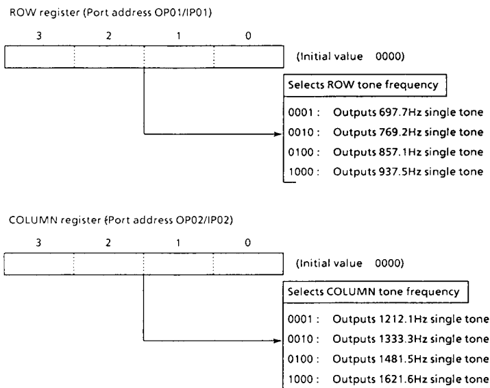
Figure 3-6. ROW, COLUMN Register
