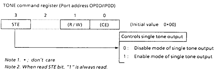
Figure 3-5. TONE Command Register
