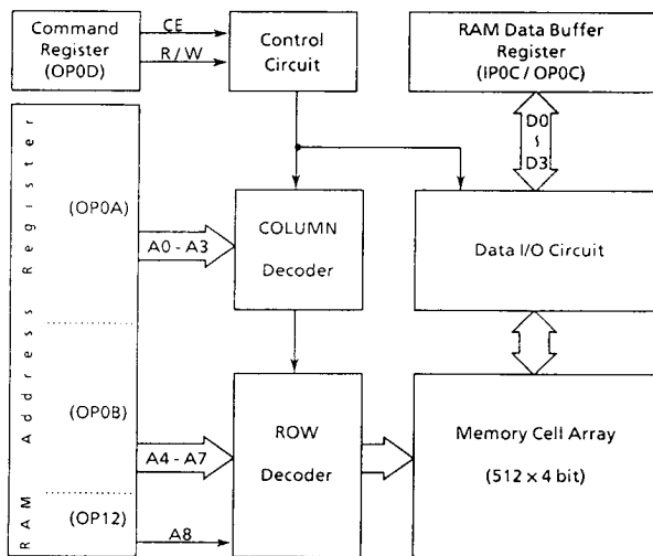
Figure 2-1. Block Diagram
