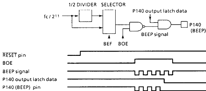
Figure 3-10. BEEP Output Circuit Configuration and Timing Chart
