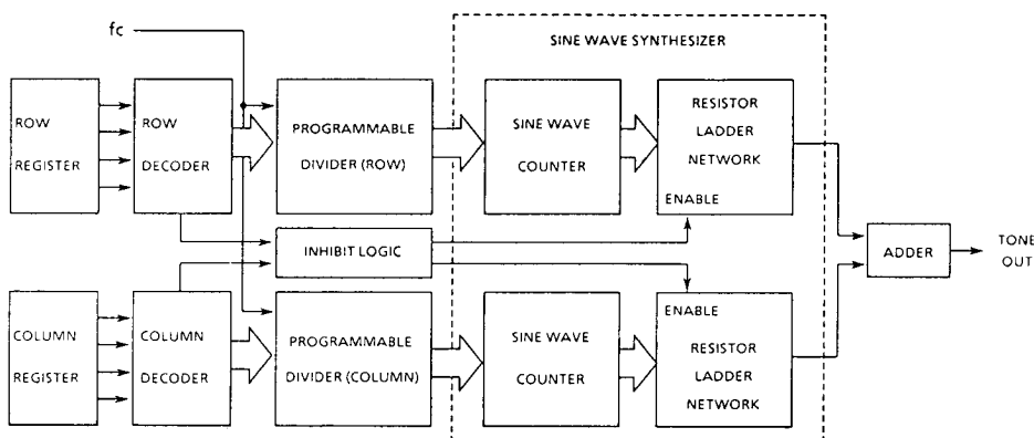
Figure 3-4. Configuration of DTMF Generator
