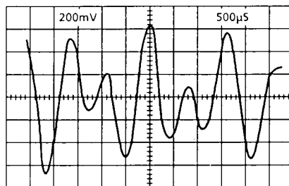
Figure 3-9. Dual tone waveform
