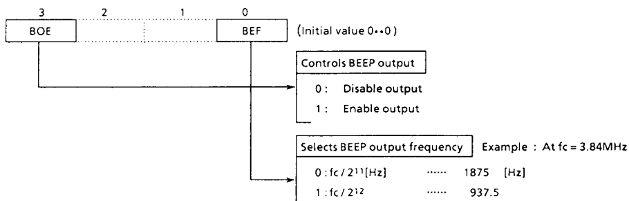
Figure 3-11. BEEP Output Control command register
