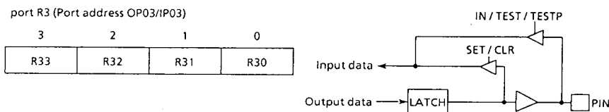
Figure 3-2. Port R3
