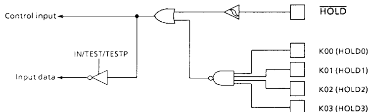
Figure 4-1. Hold control circuit
