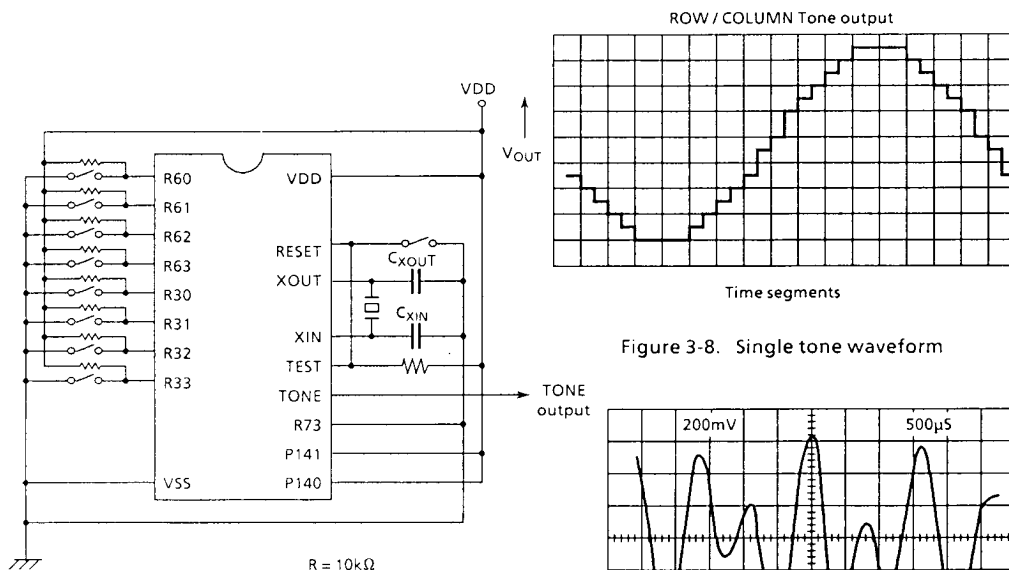
Figure 3-7. Tone test circuit
