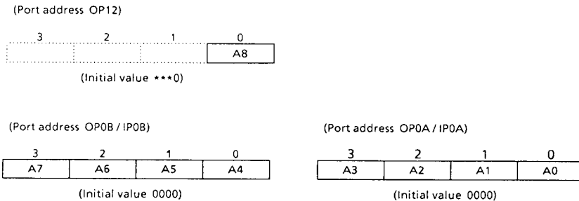
Figure 2-2. RAM Address Register
