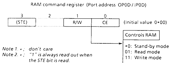
Figure 2-4. RAM Command Register
