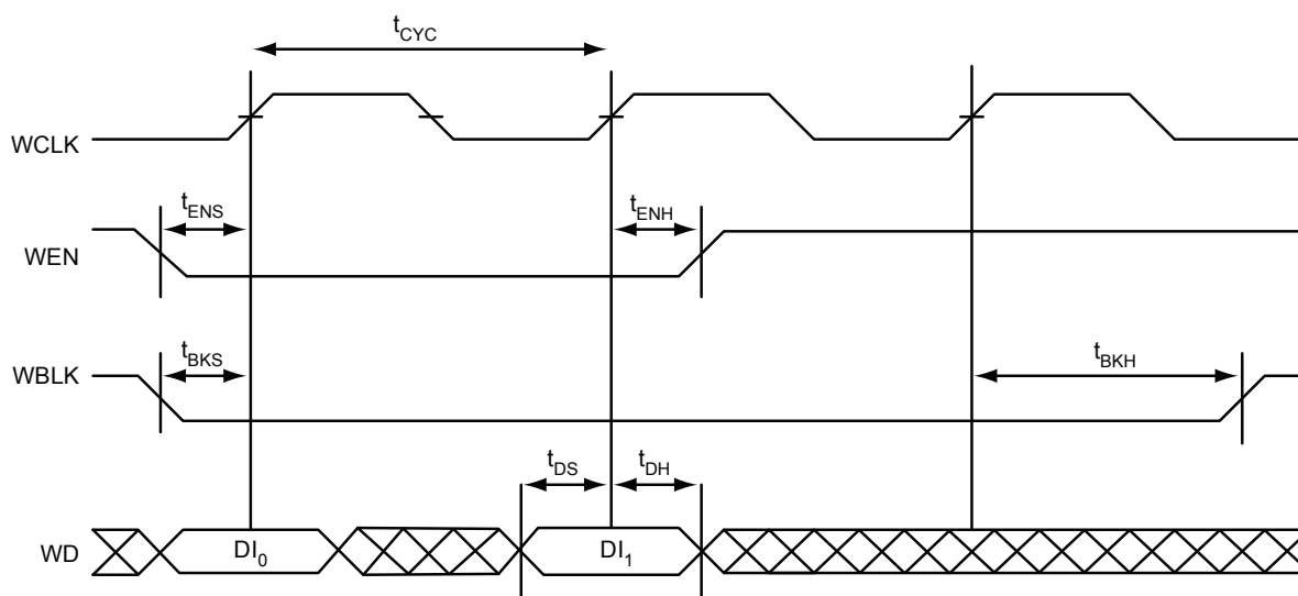
Figure 2-39 • FIFO Write
