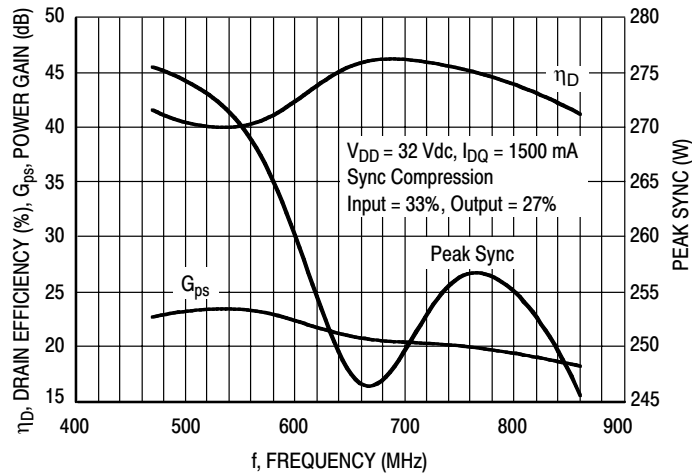
Figure 52. Peak Sync, Power Gain and Drain Efficiency versus Frequency
