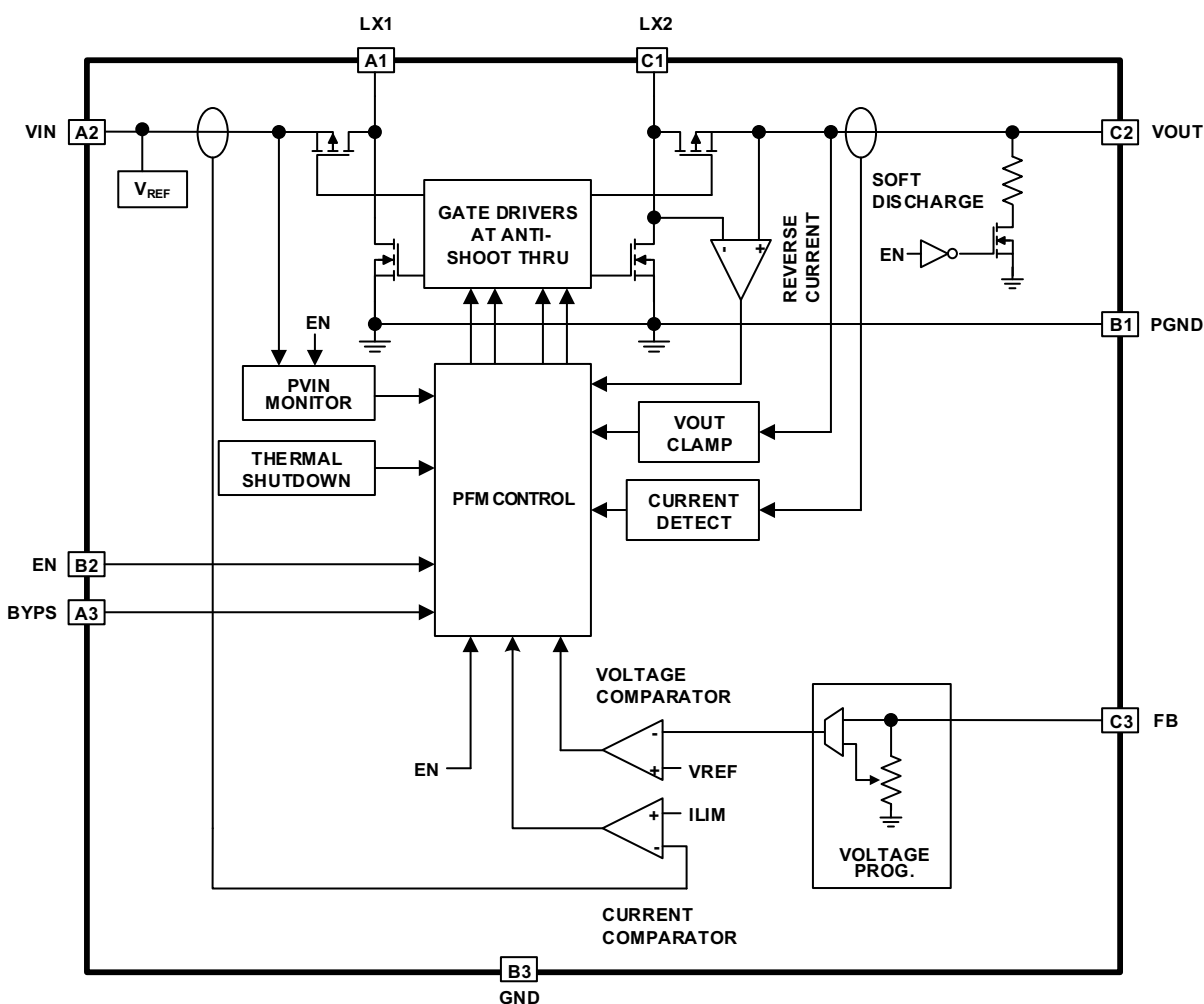
FIGURE 3. BLOCK DIAGRAM
