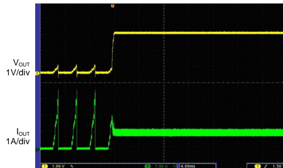
Short Circuit Recovery ( V_{IN}=3.3V , V_{OUT}=2.5V )
