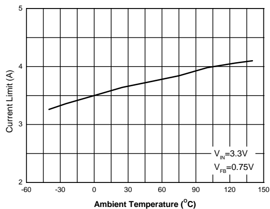
Current Limit vs. Ambient Temperature
