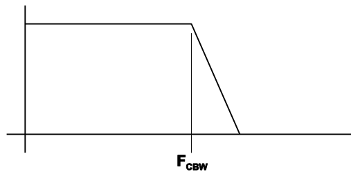
Butterworth Low-pass Filter for FSK
