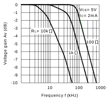
Fig.12 Frequency Response
