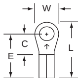
12-6S Stud Size 6 Wire Range 16-14
