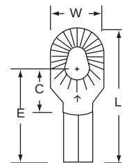
13-610 Stud Size Wire Range 6, 8, 10 12-10
