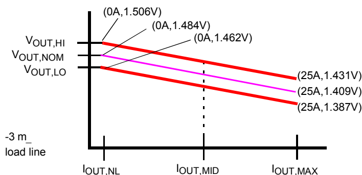
FIGURE 11. IMVP-IV ACTIVE MODE STATIC LOAD LINE
