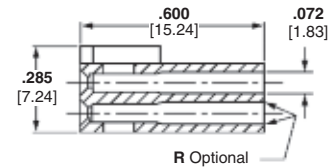
Section X-X
