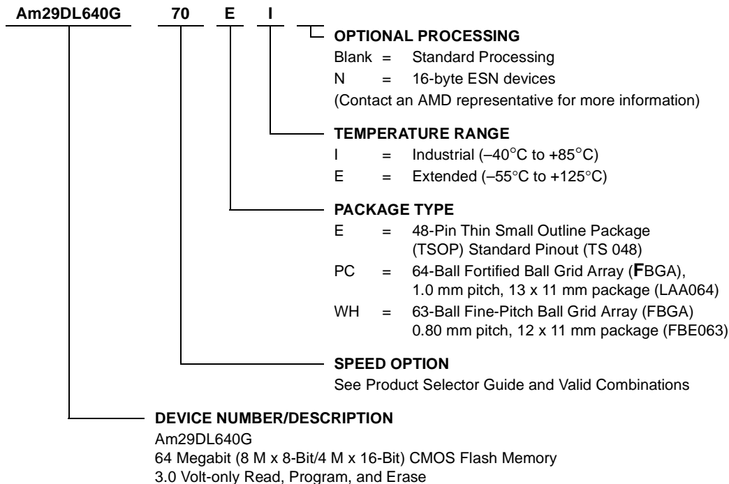
Valid Combinations for TSOP Packages
