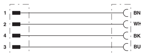
Contact assignment of M12 connector/socket
