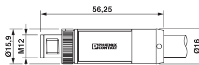
Dimensional drawing
