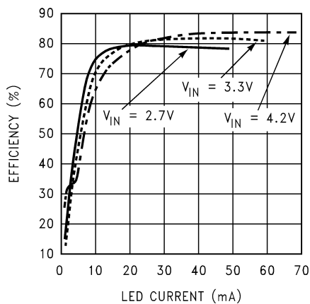
3 LED Efficiency vs LED Current
