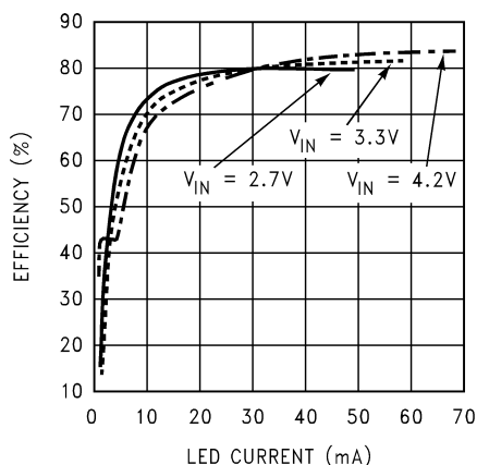
3 LED Efficiency vs LED Current
