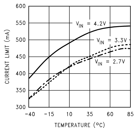
Switch Current Limit vs Temperature LM3500-16, V_{OUT}=8V
