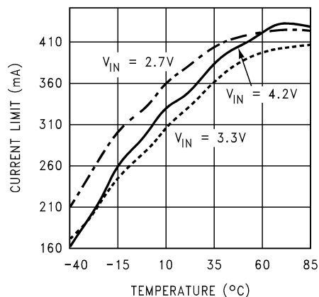
Switch Current Limit vs Temperature LM3500-16, V_{OUT}=12V
