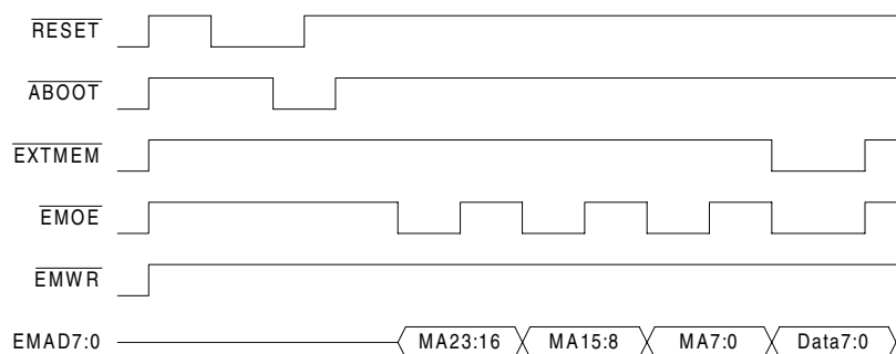
Figure 35. Autboot Timing Diagram
