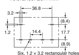
PCB Mounting Holes
