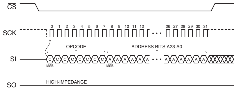
Figure 8-5. Block Erase
