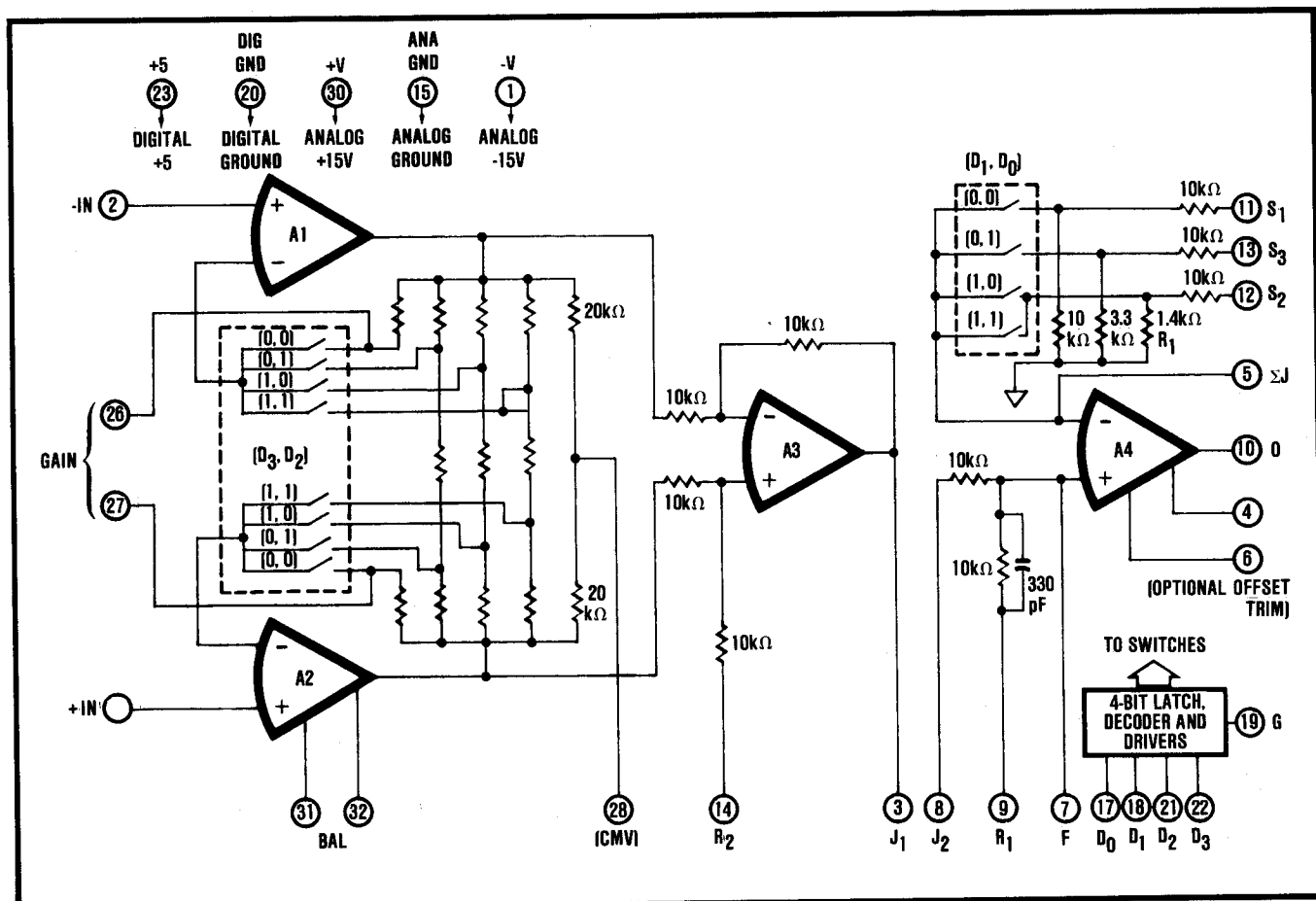
FIGURE 1. Simplified Schematic.
