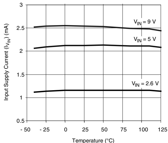
I_{VIN} (Active - Switching) vs. Temperature
