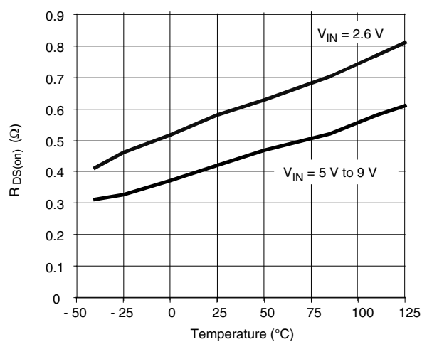
Switching On Resistance vs. Temperature
