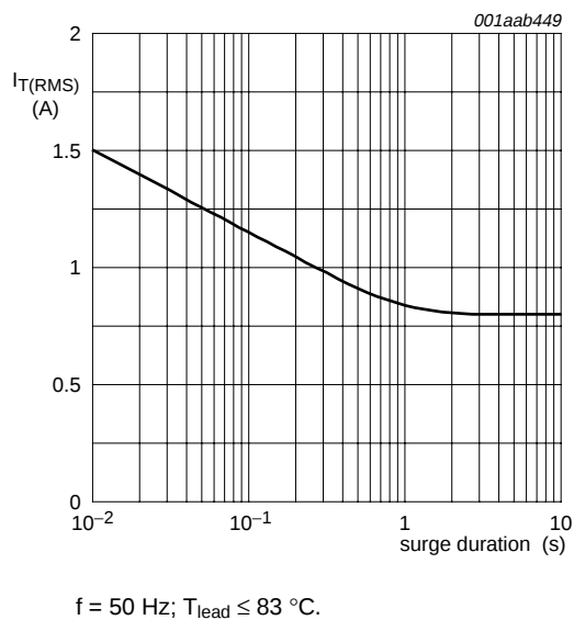
Fig 4. RMS on-state current as a function of surge duration for sinusoidal currents.
