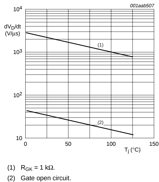
Fig 12. Critical rate of rise of off-state voltage as a function of junction temperature; typical values.
