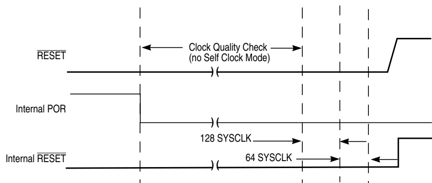
Figure 2-27. \overline{\text{RESET}} Pin Held Low Externally
