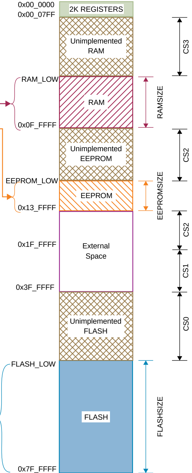
Figure 1-3. S12X CPU & BDM Global Address Mapping
