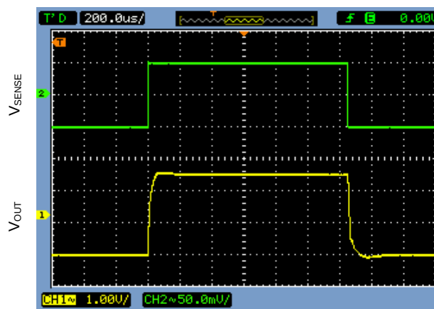
Large-Signal Pulse Response, Gain = 25
