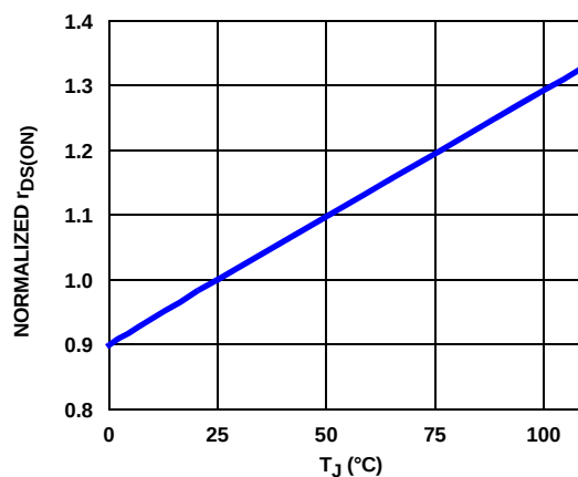
FIGURE 4. HIGH-SIDE r DS(ON) vs T J NORMALIZED FOR T J = +25 °C (V DDS = 12V, BST - SW = 6.5V, I DRAIN = 0.3A)
