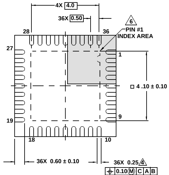
BOTTOM VIEW
