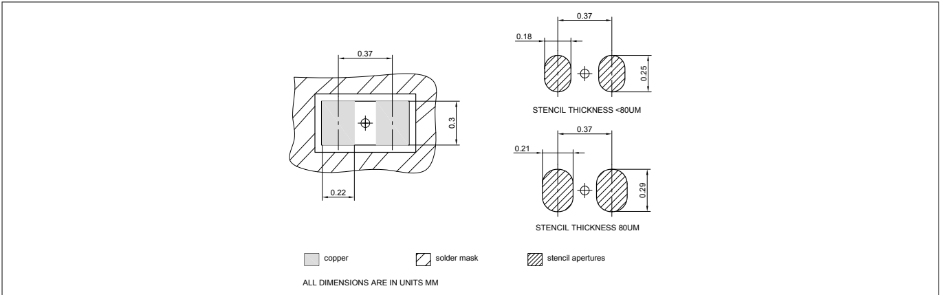
Figure 13 WLL-2-3 footprint (dimension in mm), recommendation for Printed Circuit Board Assembly see [2]
