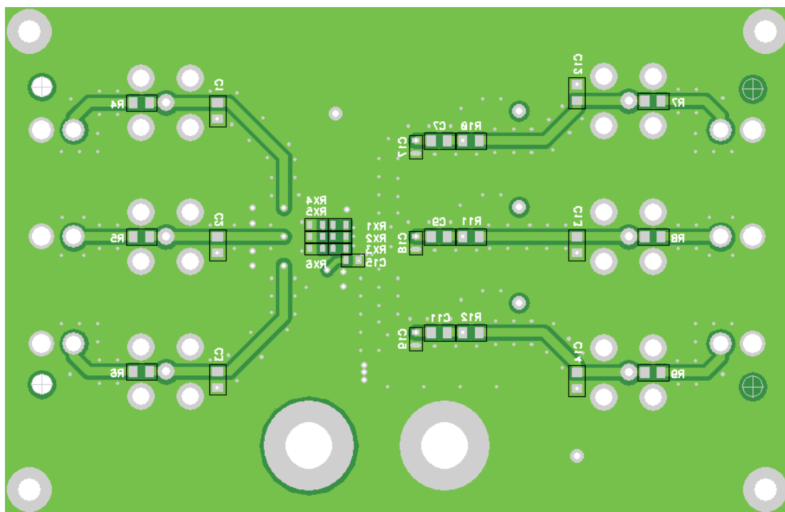
Figure 37. Bottom View
