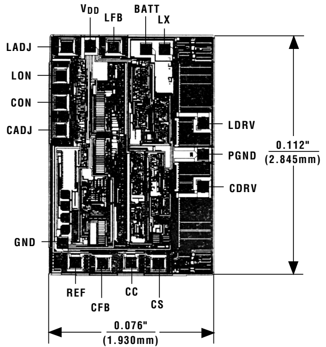
Chip Topography
