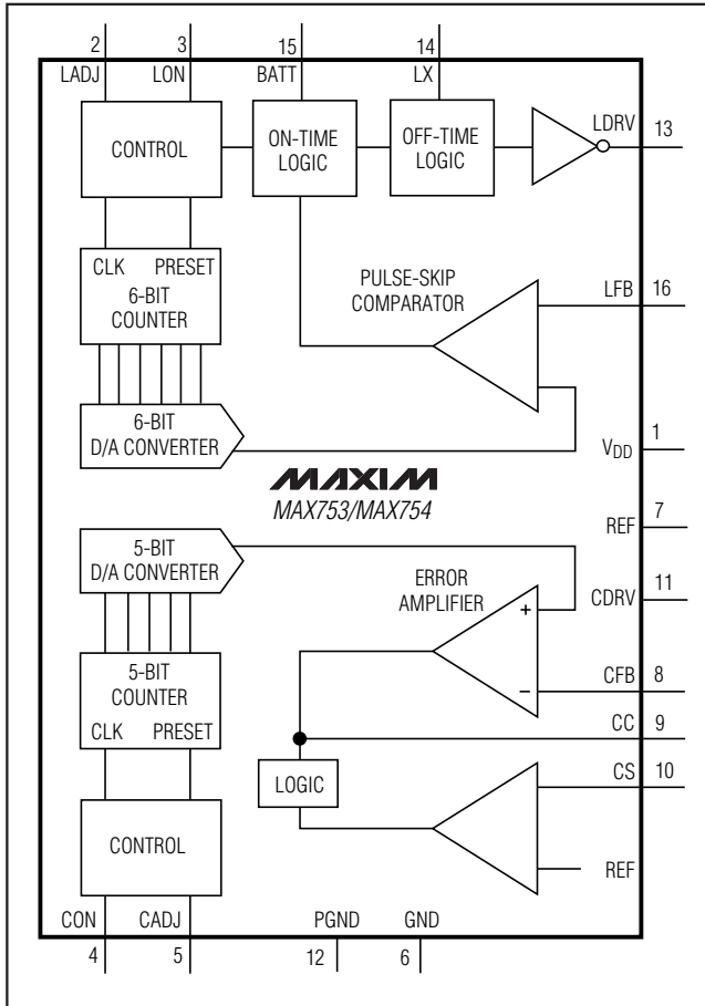
Block Diagram
