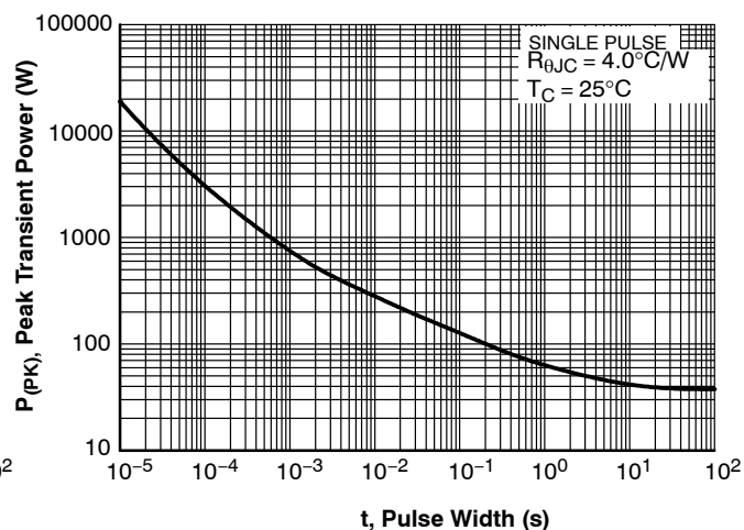
Figure 14. Single Pulse Maximum Power Dissipation for FDP4D5N10C
