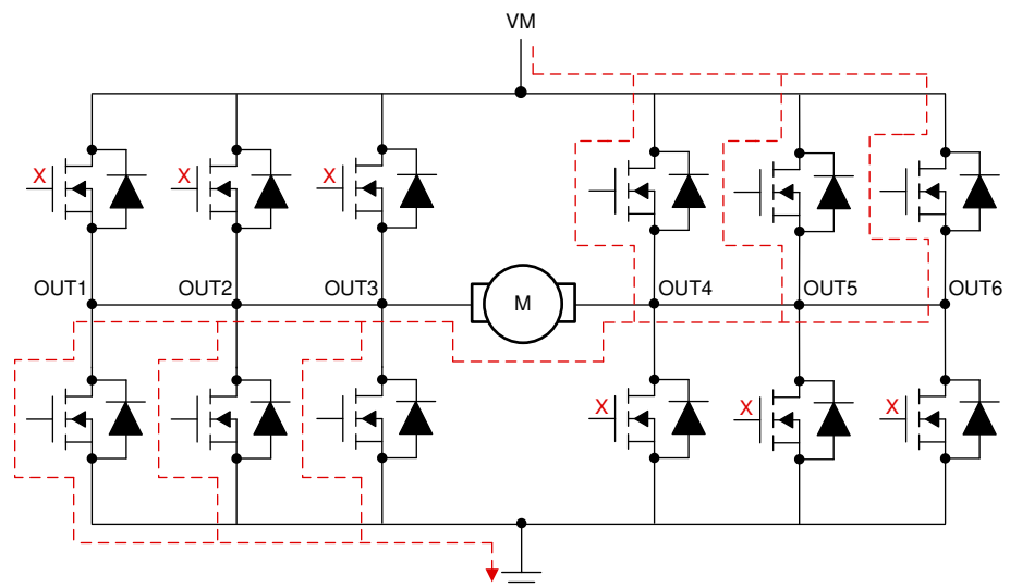
Figure 39. Parallel Mode (Reverse Direction)
