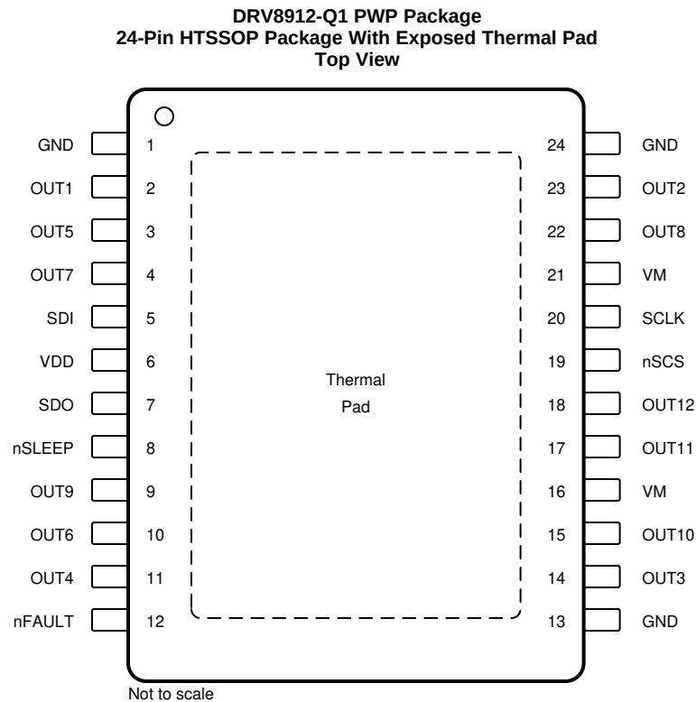
Pin Functions—DRV8912-Q1
