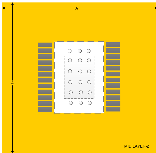
Figure 151. PCB - Mid Layer-2 (4-Layer PCB)
