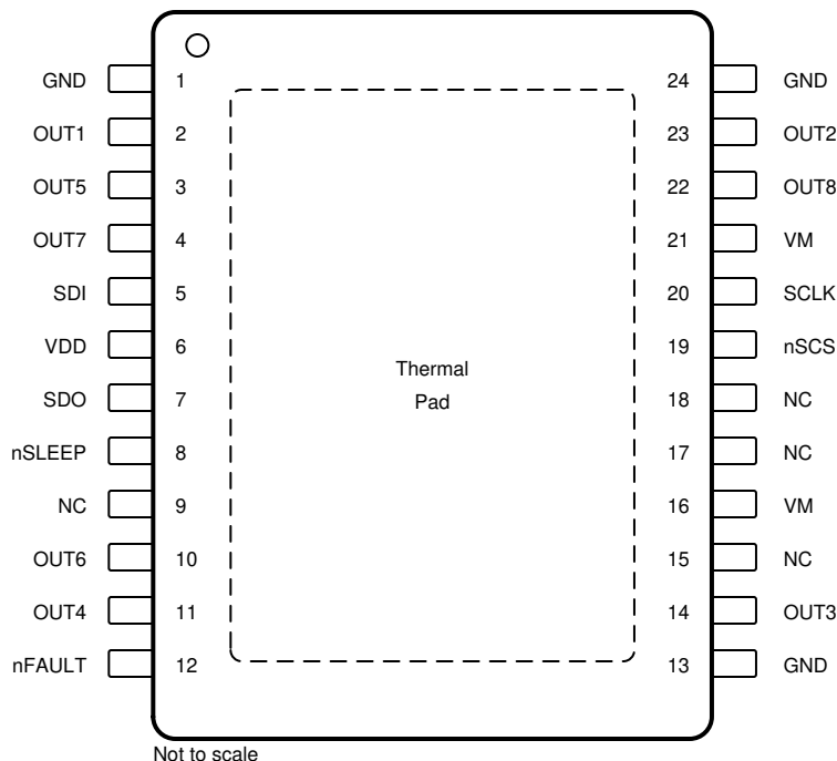
DRV8908-Q1 PWP Package 24-Pin HTSSOP Package With Exposed Thermal Pad Top View
