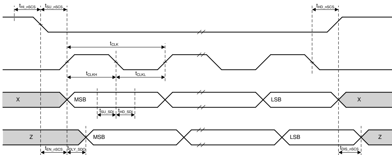
Figure 1. SPI Timing
