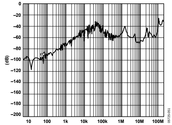
Figure 47. ADR121/ADR125/ADR127 PSRR
