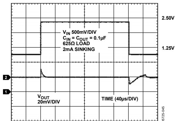
Figure 41. ADR127 Load Transient Response (Sinking)
