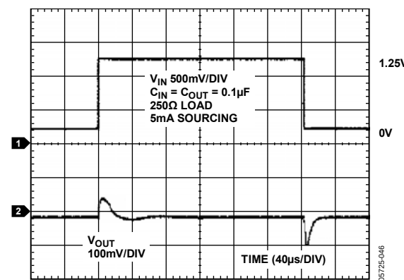
Figure 42. ADR127 Load Transient Response (Sourcing)
