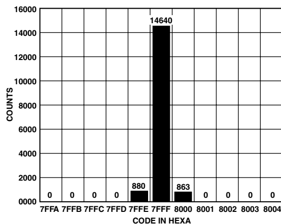
TPC 4. Histogram of 16,384 Conversions of a DC Input at the Code Center
