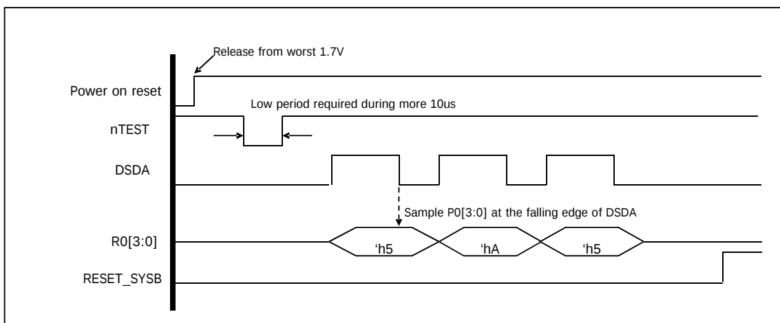
Figure 15-9 Byte-parallel mode
