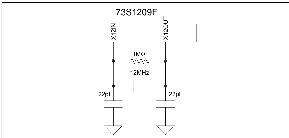
Figure 4: Oscillator Circuit
