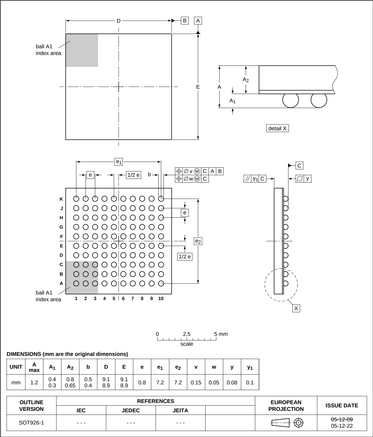
Fig 49. Package outline of the TFBGA100 package
