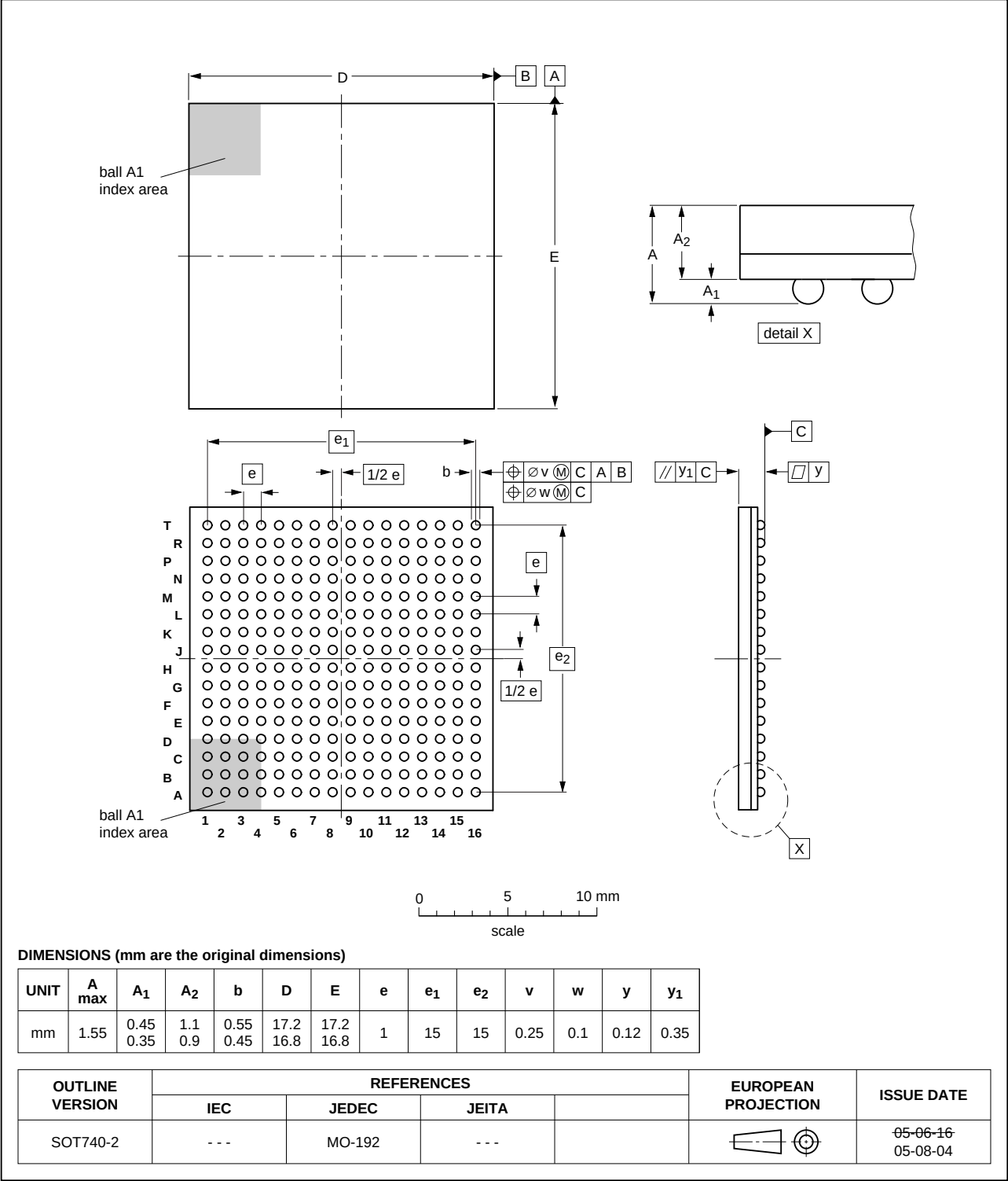
Fig 48. Package outline of the LBGA256 package
