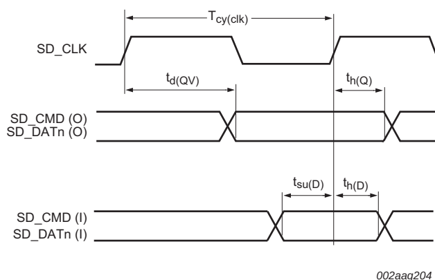
Fig 36. SD/MMC timing
