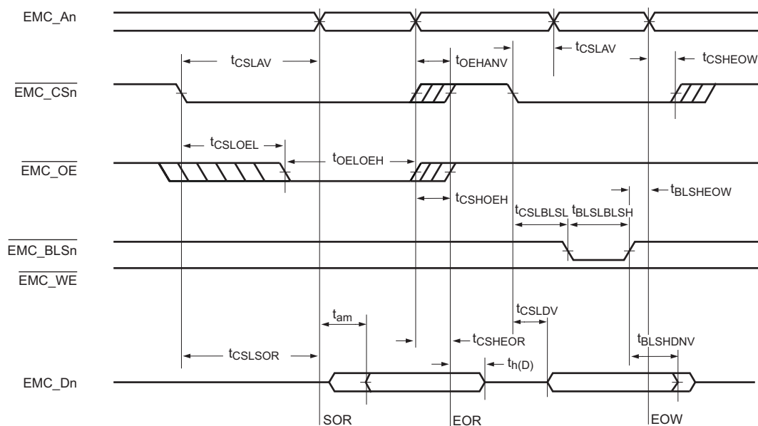
Fig 31. External static memory read/write access (PB = 0)
