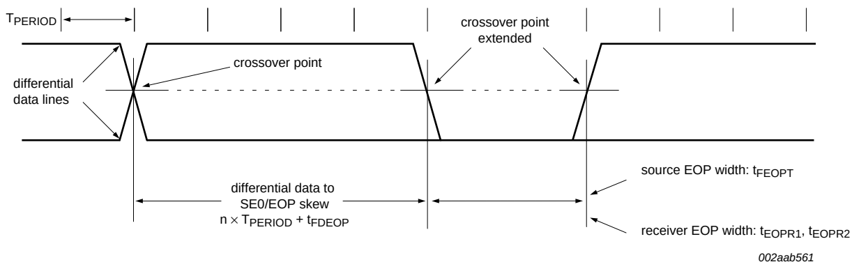
Fig 34. Differential data-to-EOP transition skew and EOP width
