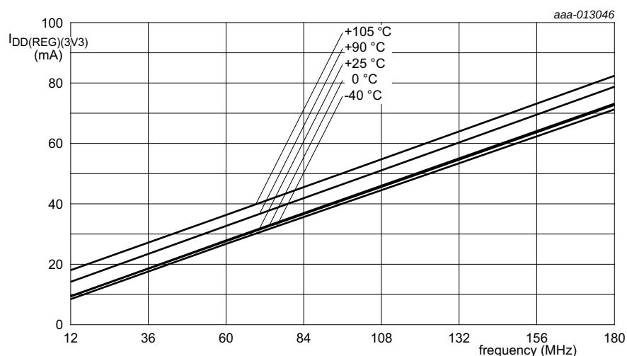
Fig 12. Typical supply current versus core frequency in active mode; code executed from SRAM
