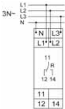
Wiring E236-US 1.1 and US 2.1
