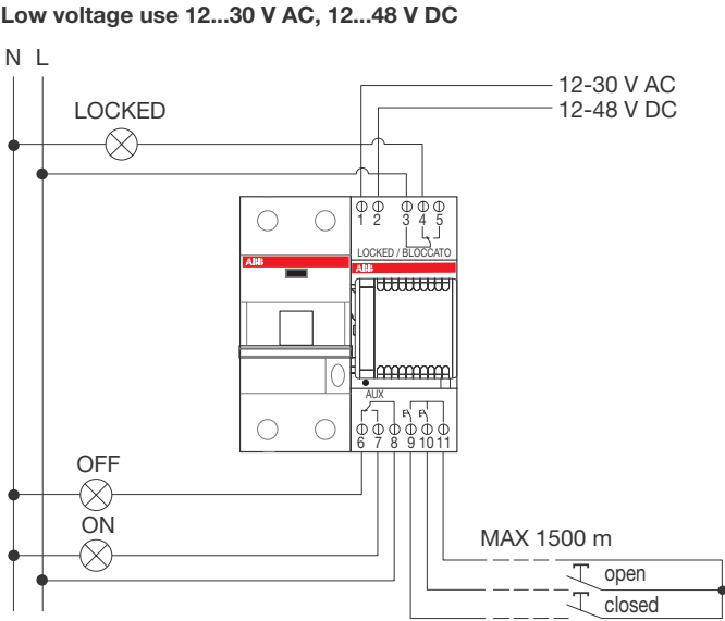
Wiring diagrams for DS2C-CM motor operating devices
