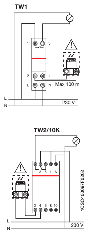
Connection diagram
