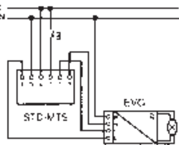
Brightness control of a fluorescent lamp with 1 - 10 V DC control input with memory touch controller STD-MTS with external pushbutton, e.g. E 225
