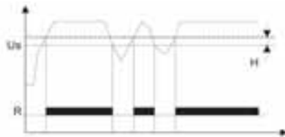
Function E236-US 1.1 and US 2.1
