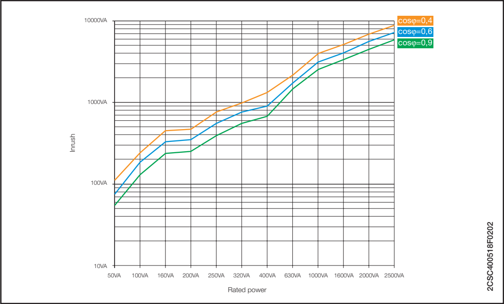
Inrush power trend
