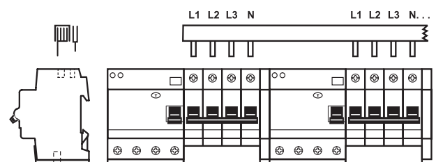
PS 4/36/16 H-DDA 204 T DS 204 ( \leq 40 A) + S2C-S/H6R + DS 204 ( \leq 40 A) + S2C-S/H6R + DDA 204 ( \leq 40 A) + S 204 + S2C-S/H6R + DDA 204 ( \leq 40 A) + S 204 + S2C-S/H6R
