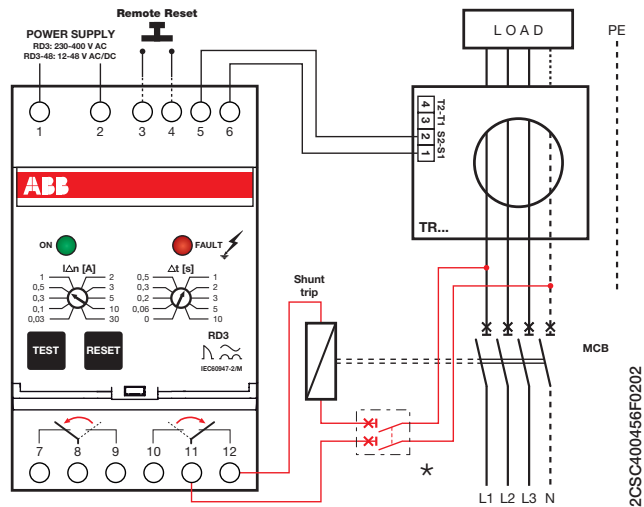
Connection with shunt trip when the current is activated
