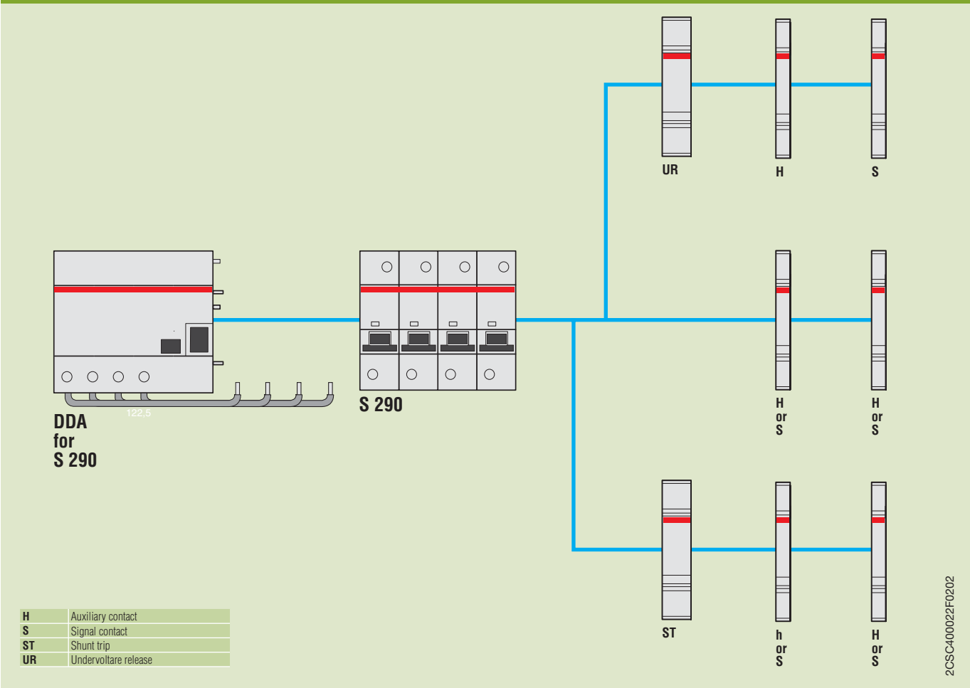
Combination between auxiliary elements and S 290
