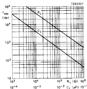
Fig. 9 RC oscillator frequency as a function of R_t and C_t at V_{CC} = 2.0 to 6.0 V; T_{amb} = 25^\circ\text{C} .
