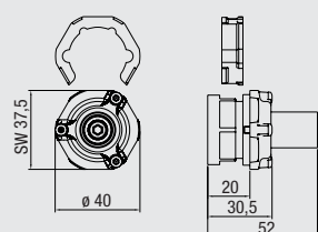
Erdkontakt Buchse Contact for grounding female
