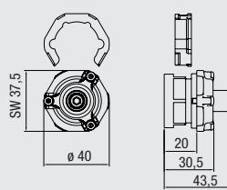
Erdkontakt Stift Contact for grounding male
