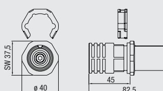
Powerkontakt Buchse Contact for power female
