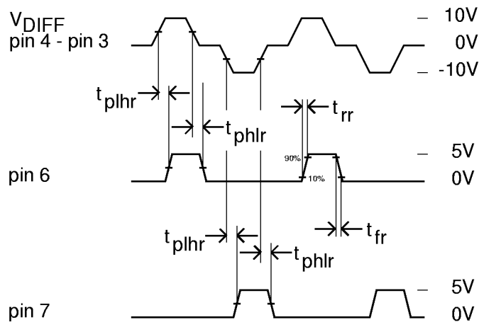
FIGURE 3 - RECEIVER TIMING
