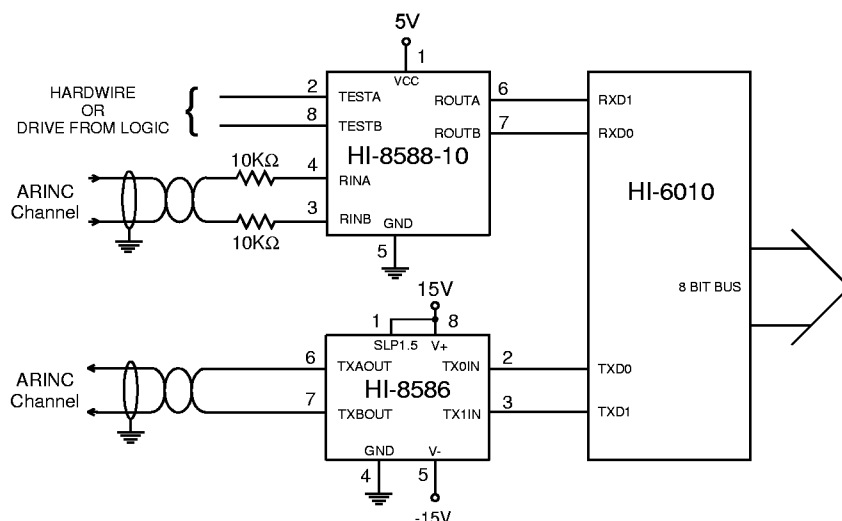
FIGURE 2 - APPLICATION DIAGRAM
