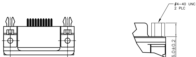
DETAIL Z (W/SCREWLOCKS OPTION)
