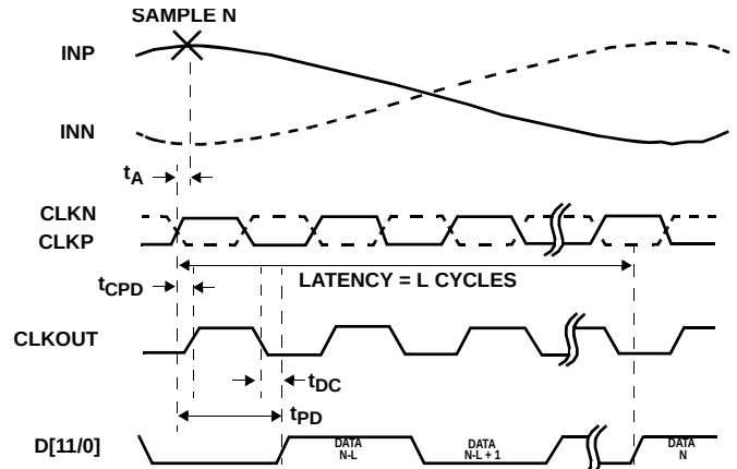
FIGURE 2B. SDR
