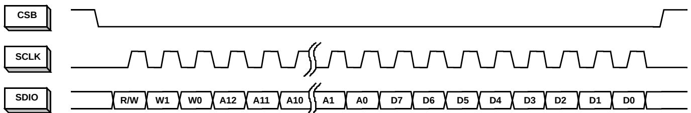
FIGURE 33. MSB-FIRST ADDRESSING
