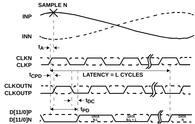
FIGURE 1B. SDR
