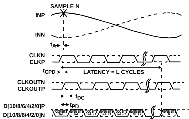
FIGURE 1A. DDR
