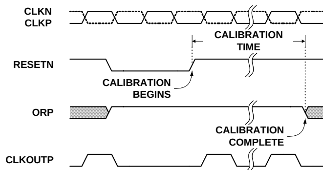
FIGURE 22. CALIBRATION TIMING
