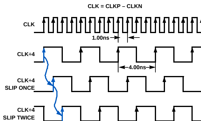
FIGURE 39. PHASE SLIP: CLK÷4 MODE, f_{\text{CLOCK}} = 1000\text{MHz}
