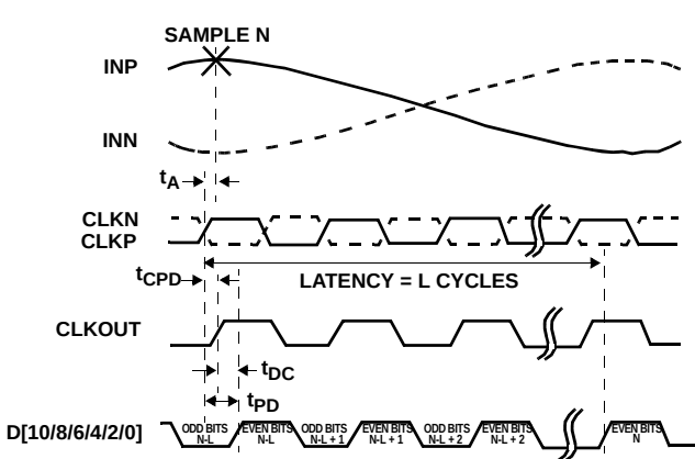
FIGURE 2A. DDR
