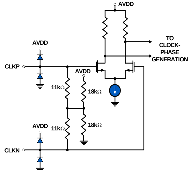
FIGURE 42. CLOCK INPUTS
