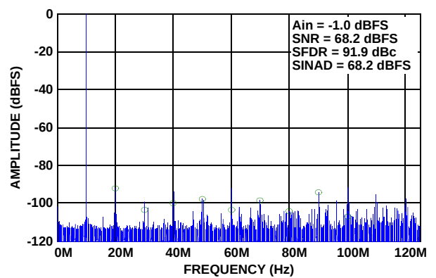
FIGURE 14. SINGLE-TONE SPECTRUM @ 10MHz
