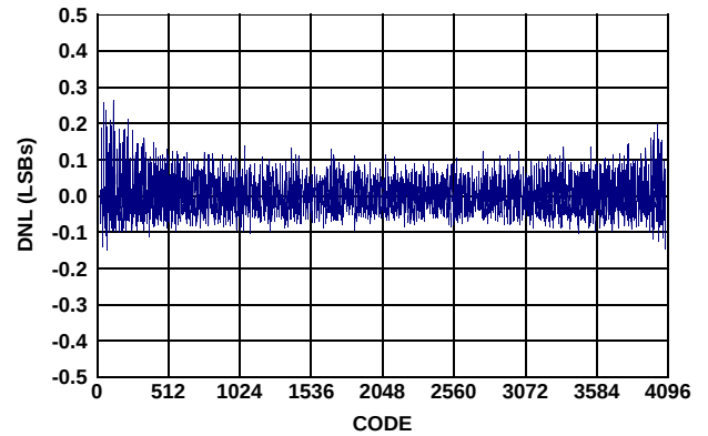
FIGURE 10. DIFFERENTIAL NONLINEARITY
