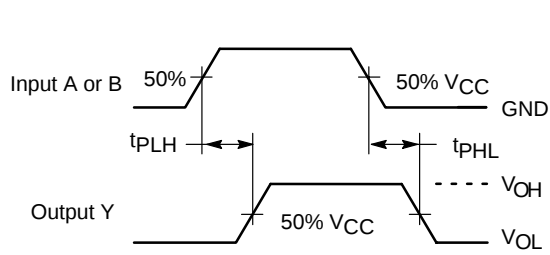
Figure 4. Switching Waveforms
