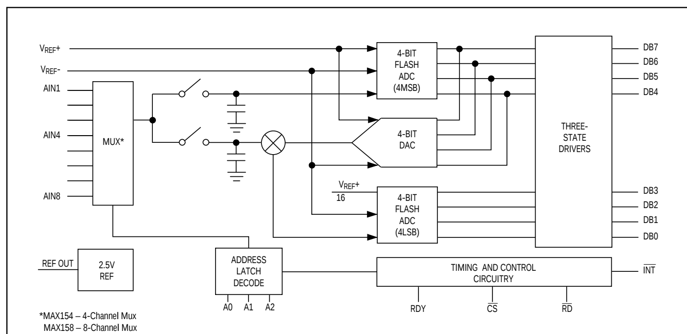
Figure 3. Functional Diagram
