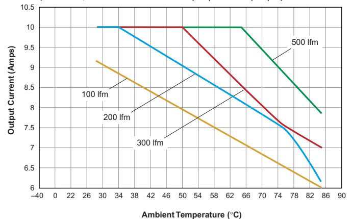
ULQ-12/10-D48 Output Current vs. Ambient Temperature ( V_{IN} = 48V , air flow direction from Input pin to Output pin)
