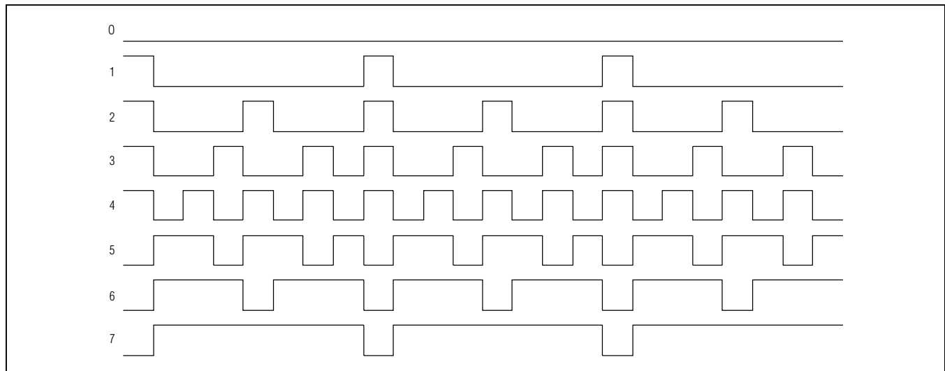
Figure 9. Delta-Sigma Output
